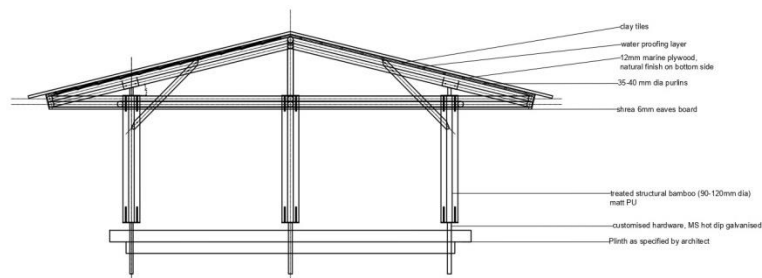
Gazebo-front elevation-diagonal plan
