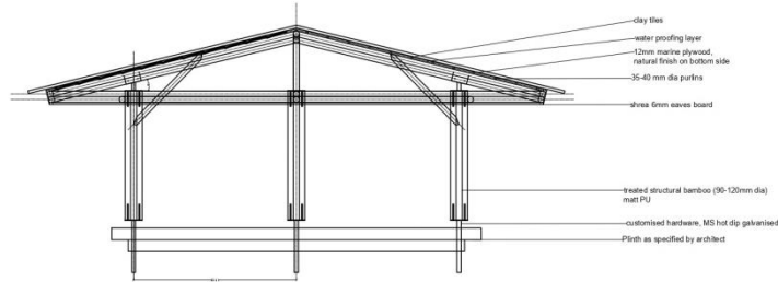
Gazebo-front elevation diagonal plan
