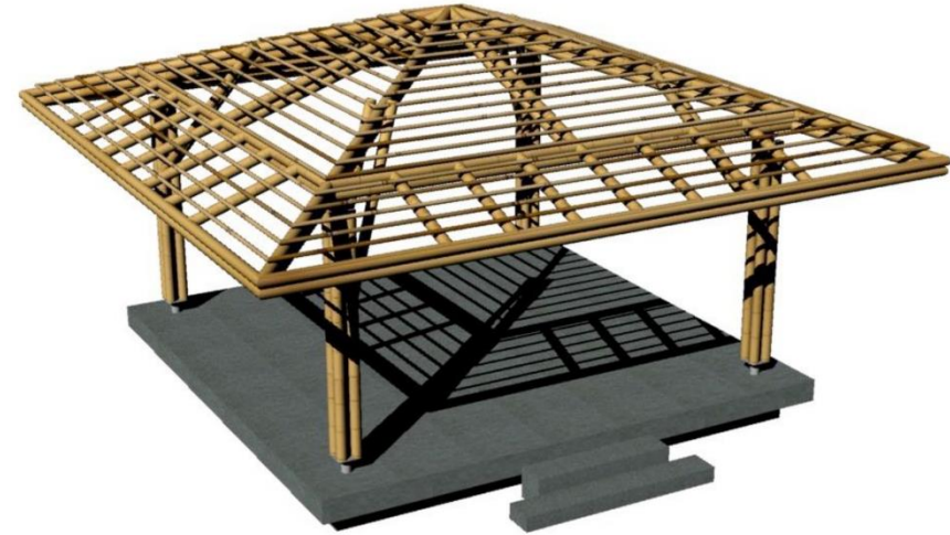
Gazebo Bajaj Officers club Bamboo structure
