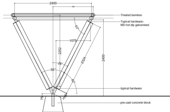
Y-Trellis-Side elevation
