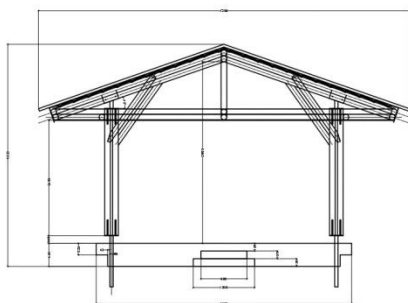
Gazebo-Front Elevation
