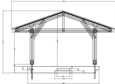
Gazebo-Front Elevation
