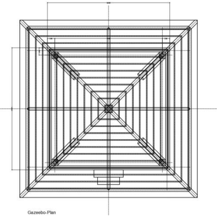
Gazebo-Plan
