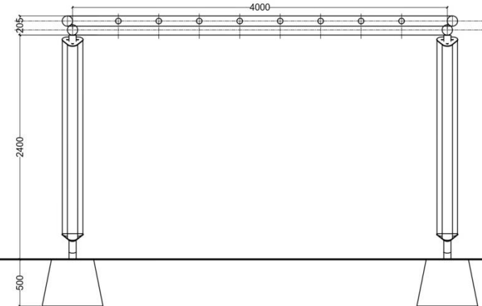
Y-Trellis-Front Elevation
